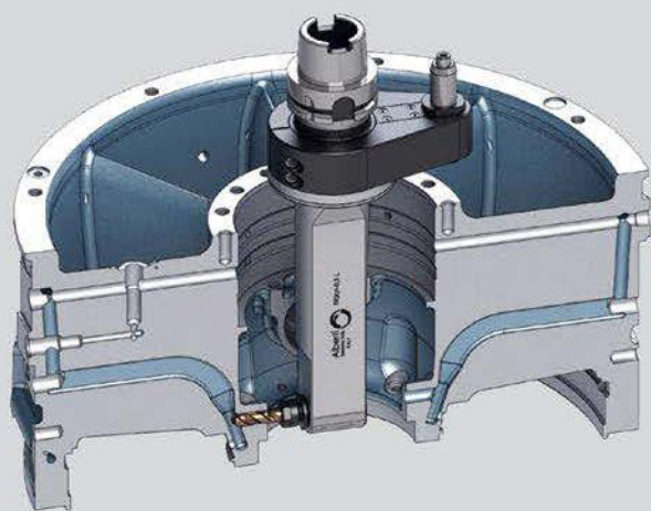
Testa a 90° prolungata 90° head with extended length
